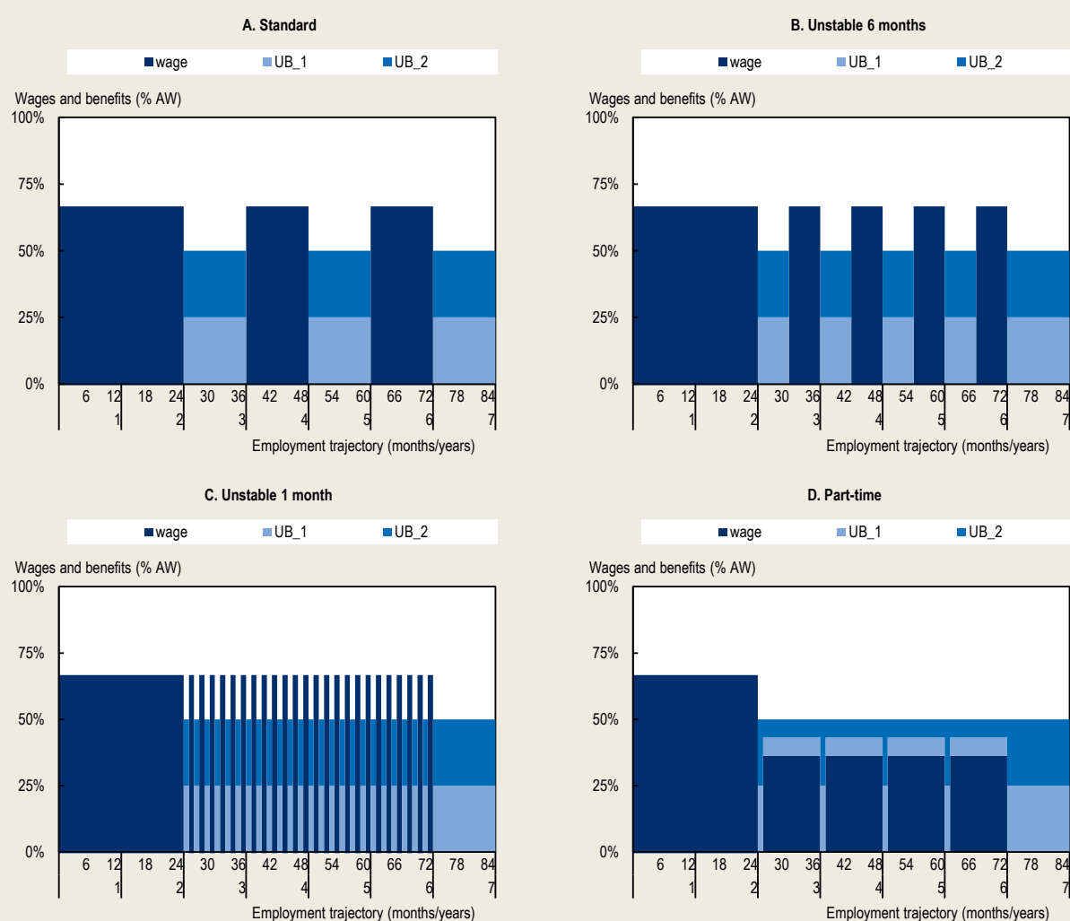
Figure 2.8. Simulation scenarios
